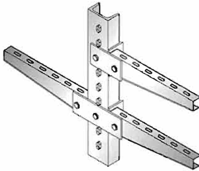
UNP SUPPORT
