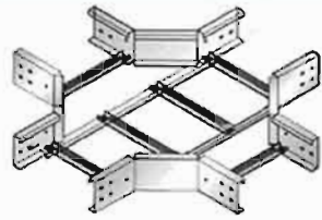
HORIZONTAL CROSS
